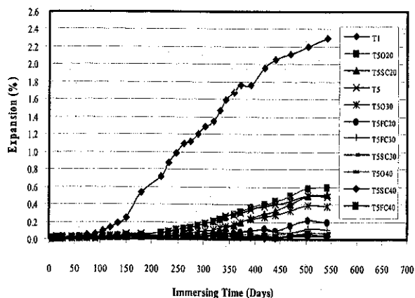
Fig 5. Expansion of Portland Cement Type V Mortar Bars Containing Fly ashes Immersed in 5% Magnesium Sulfate Solution up to 540 Days.
