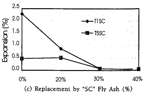
Fig 6. Relationship Between Expansion of Portland Cement Type I and Type V Mortar Bars Containing Fly Ash O, FC and SC immersed in 5% Magnesium Sulfate Solution at 540 days and Percentage of Fly Ash Replacement.
