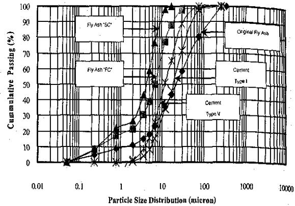
Fig 3. Particle Size Distribution of Portland Cement Type I and V and Fly Ash O, FC and SC.
