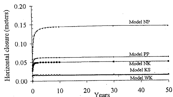
Figure 5 Horizontal closure of cavern models.
