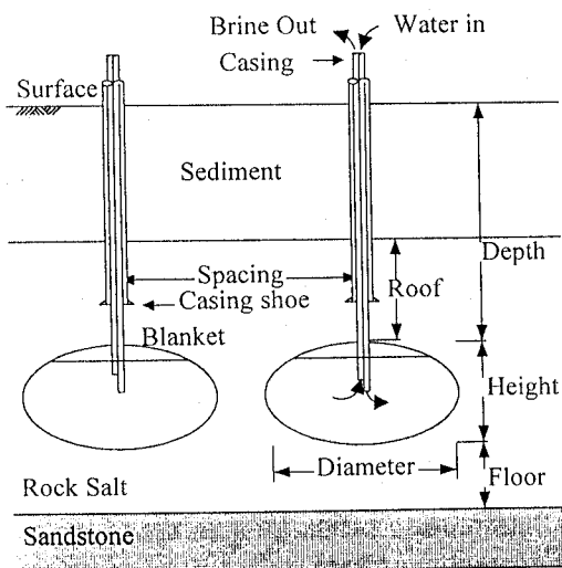
Figure 1 Design parameters for salt caverns.
