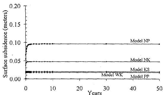
Figure 7 Surface subsidence.
